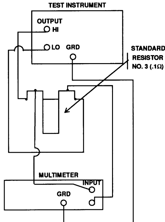
Figure 7. Dc current (1 and 2 A).
