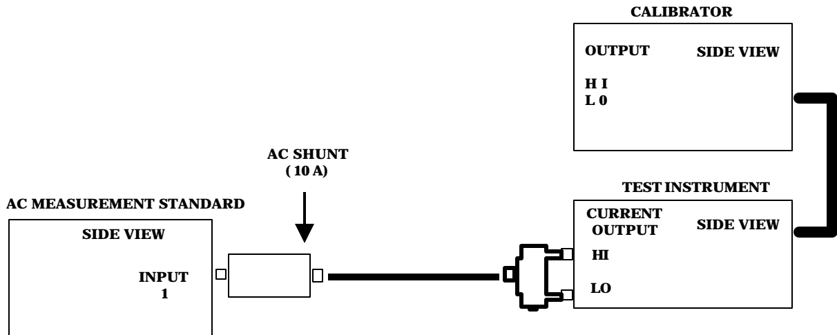
Figure 21. Frequency response.
