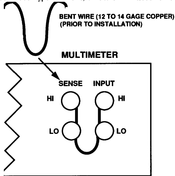
Figure 1. Four-terminal short.
